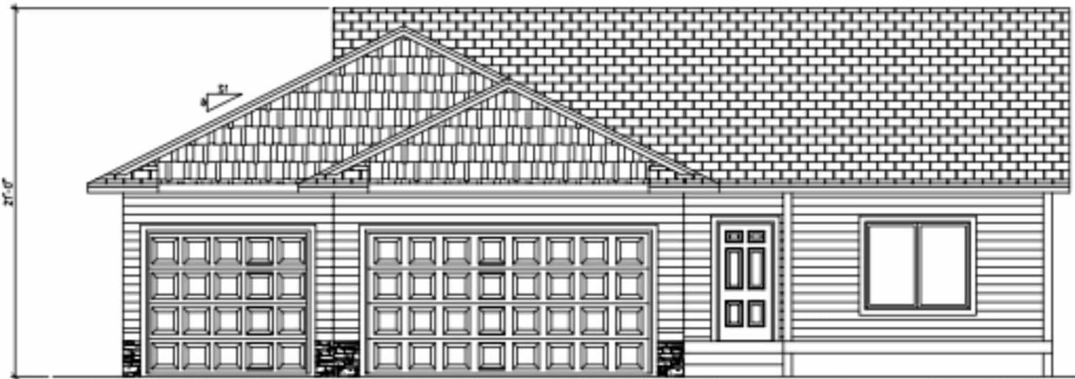
FRONT ELEVATION 1/4"=1'-0"
