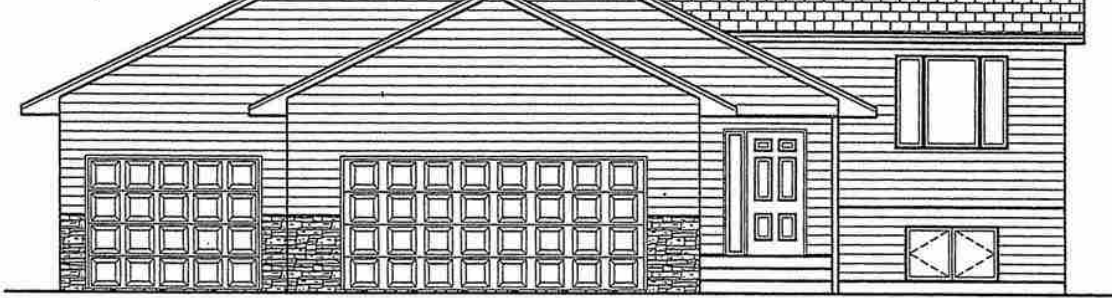
FRONT ELEVATION 1/4"=1'-0"
