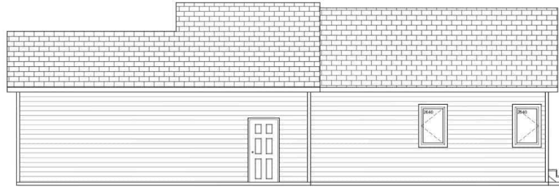
REAR ELEVATION 1/8" = 1'-0"
