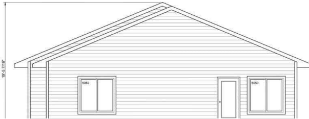
RIGHT ELEVATION 1/8" = 1'-0"
